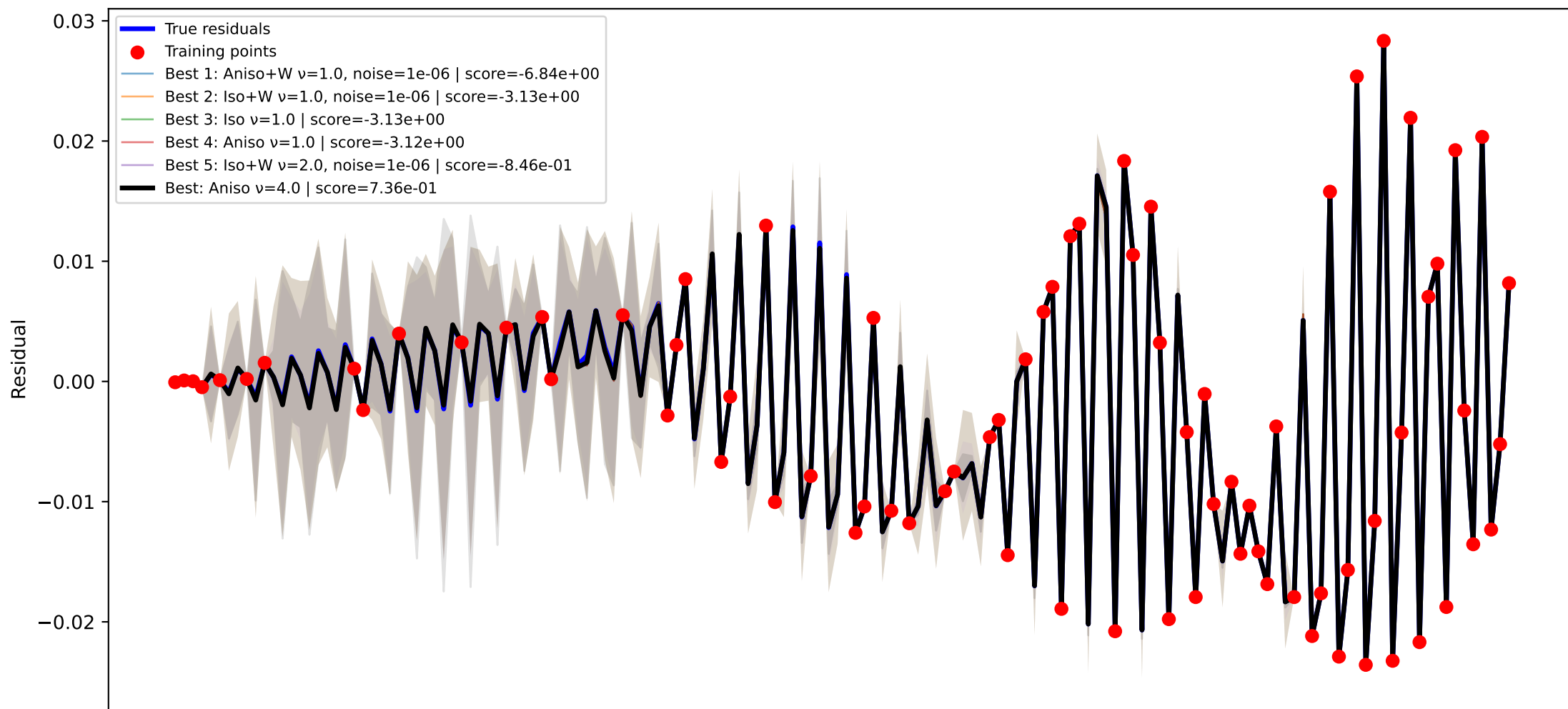
GPR kernel comparison node=30 RMSE=1.281e-04, train RMSE=3.060e-11
